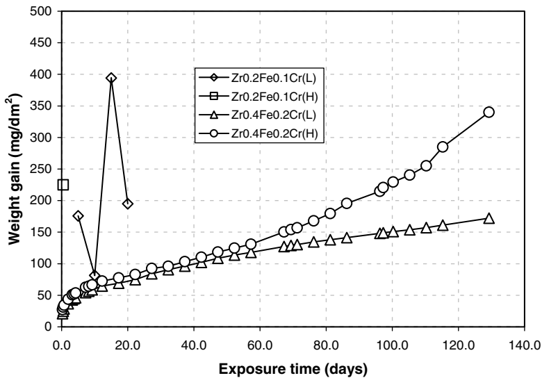
Fig. 2. Corrosion weight gain for ZrFeCr alloys in 500 °C steam.
