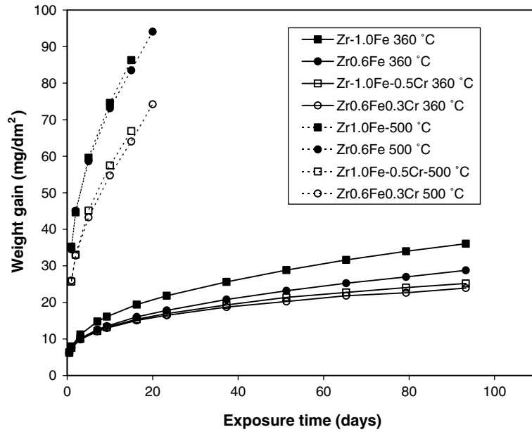
Fig. 1. Corrosion weight gain ( \text{mg}/\text{dm}^2 ) versus exposure time (days) for ZrFeCr alloys tested in 360 °C water and in 500 °C steam.
